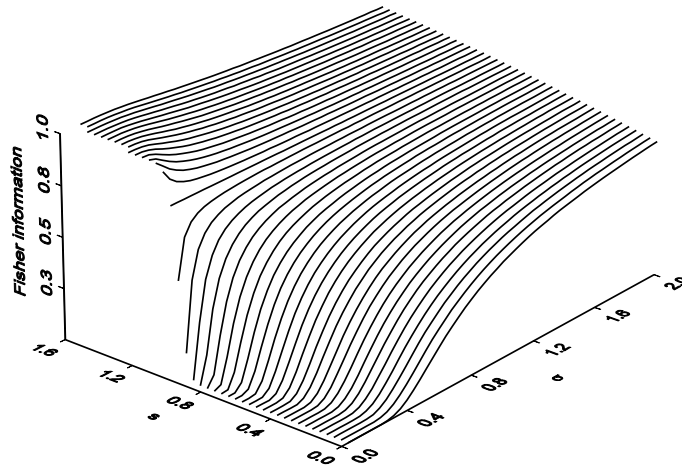
Figure 4: Proportion of information, I_{s\sigma}^{>1}/I_\sigma , retained by X_i^{>1} .
