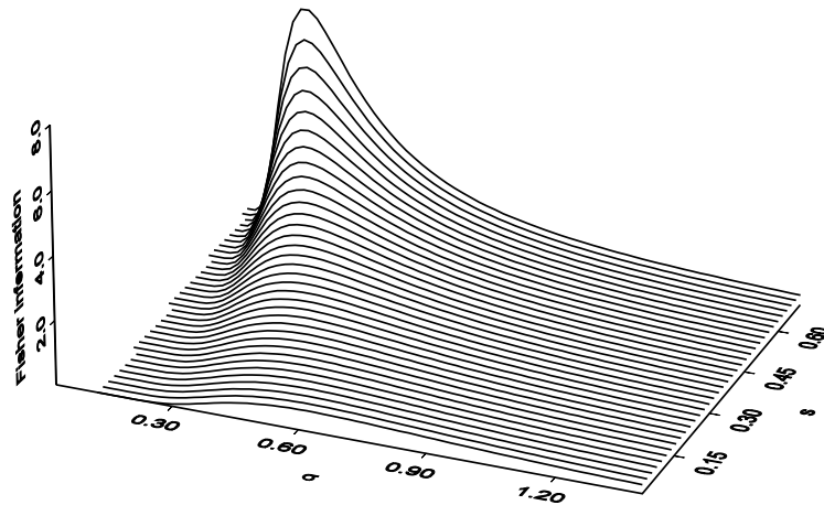
Figure 1: Fisher information I_{s\sigma}^1 .
