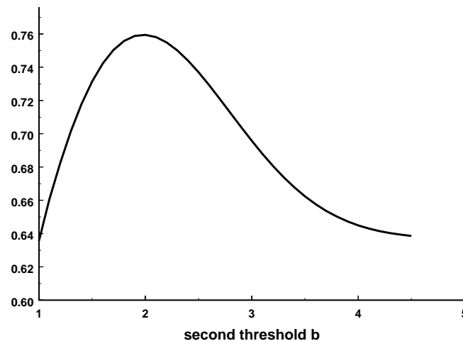
Figure 3: Proportion of information, I_{11}^{1b}/I_1 , retained by two thresholds, at 1 and b , for noise variance 1.
