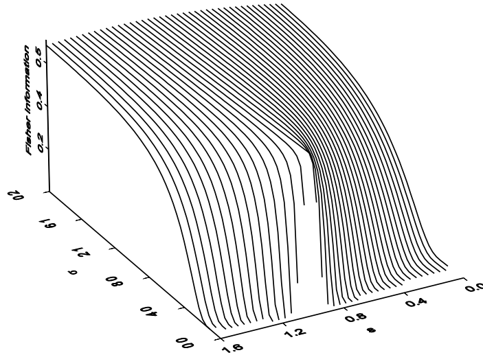
Figure 2: Proportion of information, I_{s\sigma}^1/I_\sigma , retained by X_i^1 .
